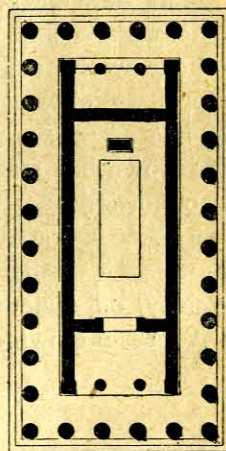
Peripter.
